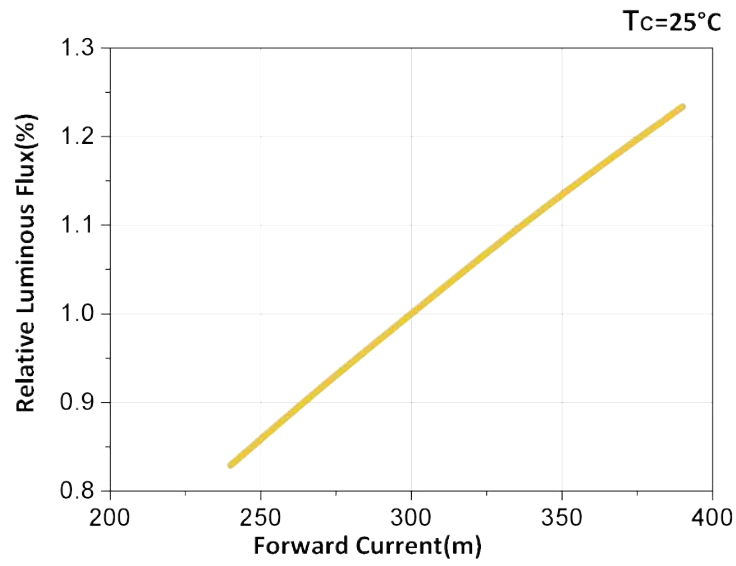
Relative Luminous Flux vs Forward Current
