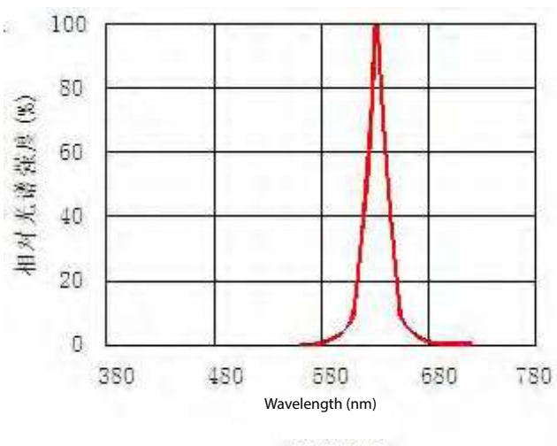
Spectrum Distribution
