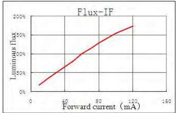
Relative Flux VS Forward Current
