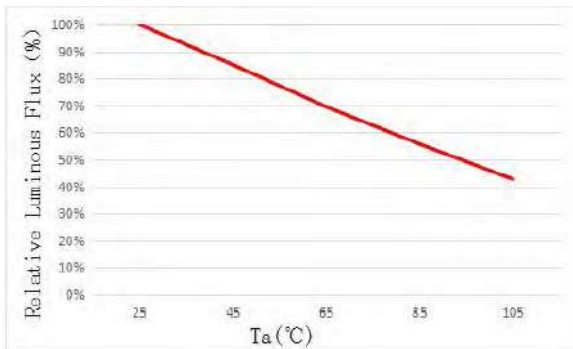
Relative Flux VS Ambient Temperature
