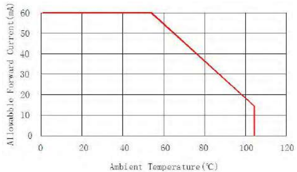
Forward Current VS Ambient Temperature
