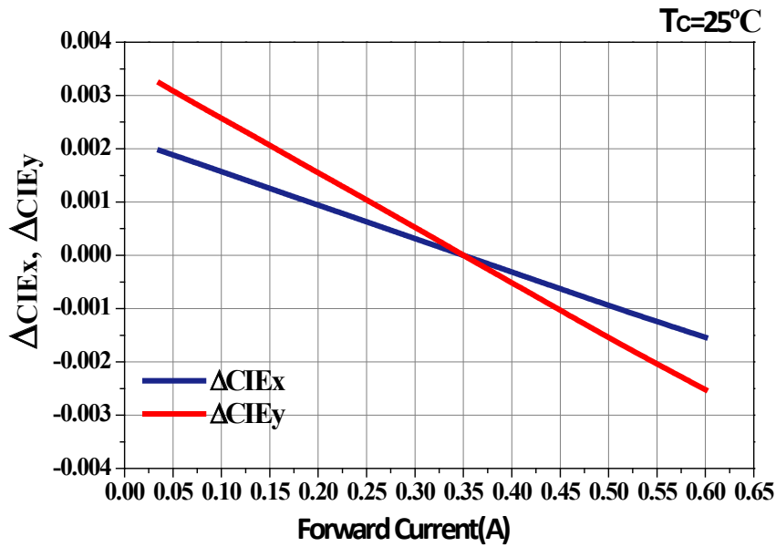
\Delta CIE x, \Delta CIE y vs Forward Current CRI(Ra)=80 Tc =25°C If= 350mA
