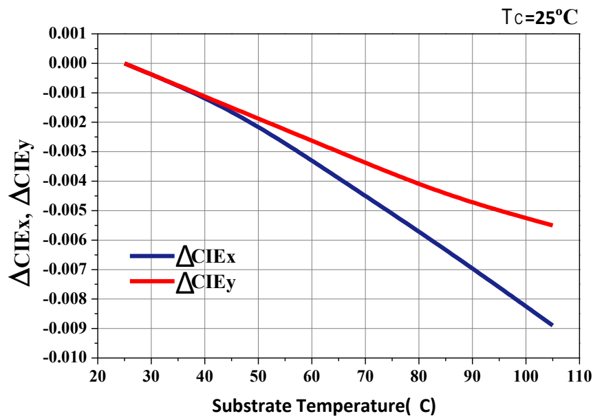
\Delta CIE x, \Delta CIE y vs Substrate Temperature CRI(Ra)=80 Tc =25°C If= 350mA
