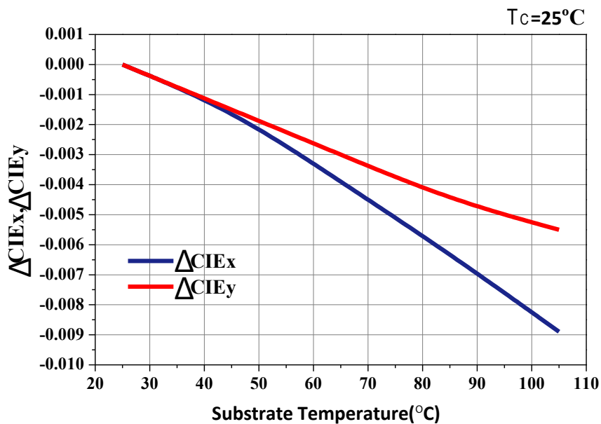
\Delta CIE x, \Delta CIE y vs Substrate Temperature CRI(Ra)=80 Tc =25°C If= 200mA
