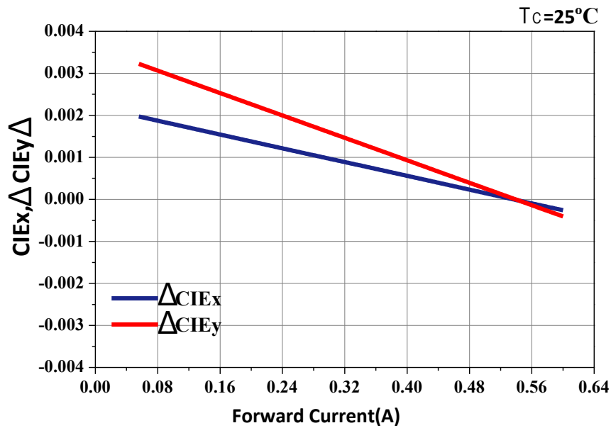
\Delta CIE x, \Delta CIE y vs Forward Current CRI(Ra)=80 Tc =25°C If= 200mA
