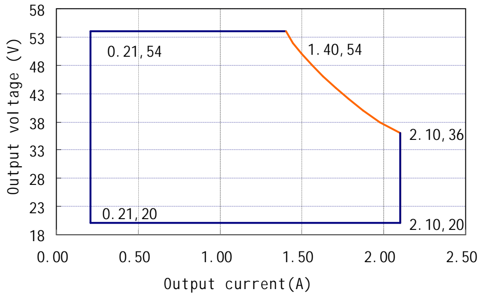
Output voltage vs Output current curve
