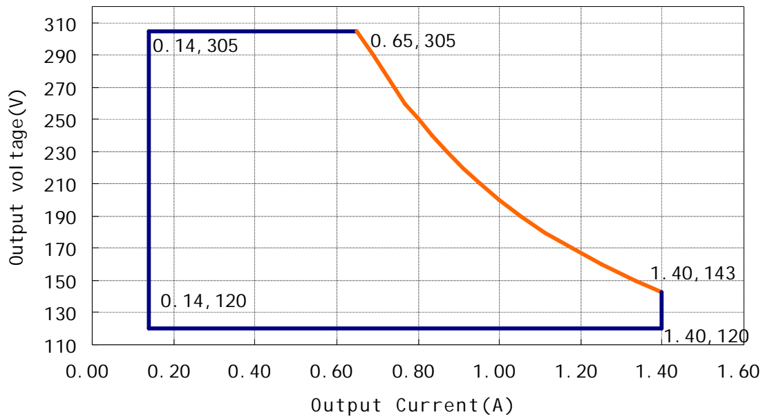
Output Voltage VS Current Curve
