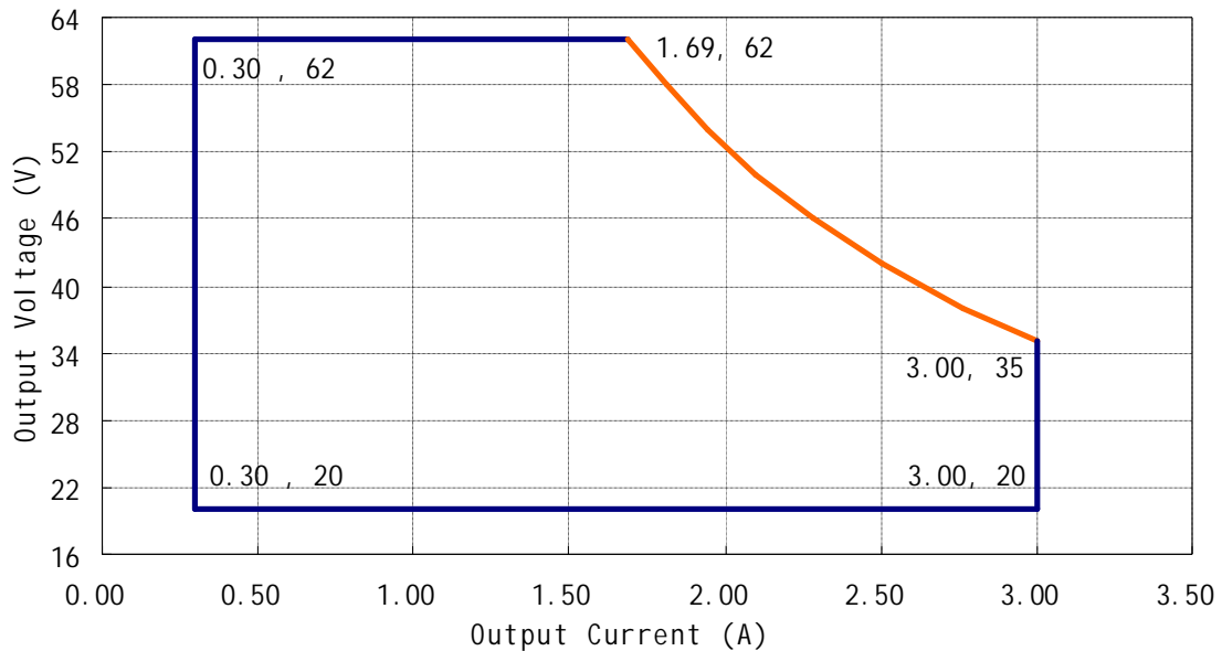
Output Voltage VS Current Curve
